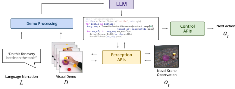
Figure 1: An overview of the SHOWTELL framework. First, the visual and spoken components of the demo are processed and fed into an LLM. The LLM synthesizes a modular program that can jointly reason about the provided demonstration and novel observations to transfer the demonstrated skill to new scenes.
